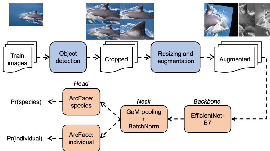
FIGURE 2 A model of the training pipeline for multi-species photo-id of cetaceans. The top row consists of preprocessing steps, shown in example by an image of a common dolphin Delphinus delphis . Crops generated by the four object detection models are shown, as well as two examples of images generated by the data augmentation step. The bottom row shows the training steps of the image classification network, from the backbone to the neck to the classification head. See Section 2 for a description of each component in the pipeline.
